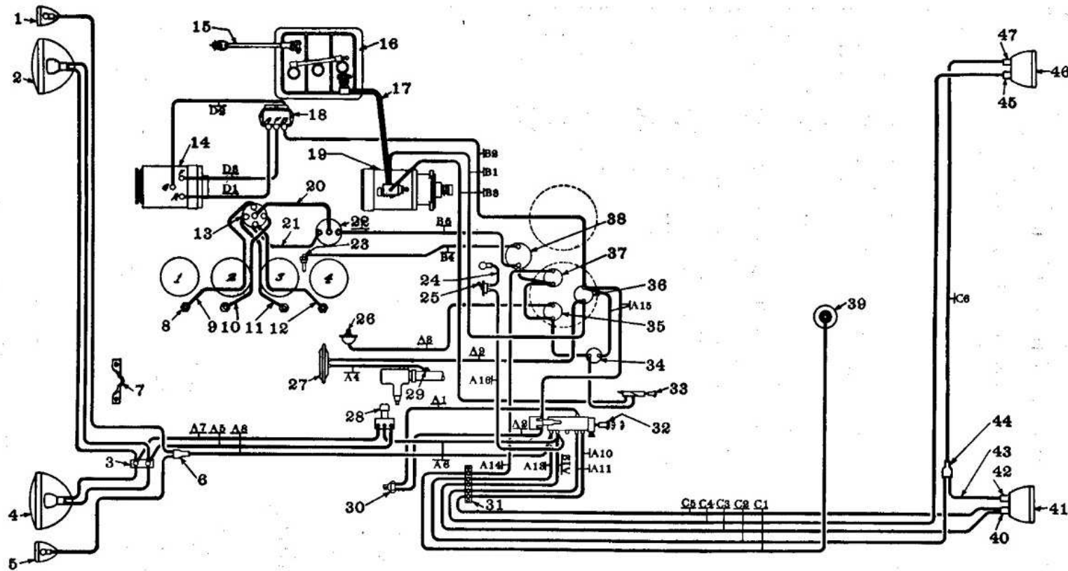
Model MA FIG. 40—WIRING DIAGRAM
